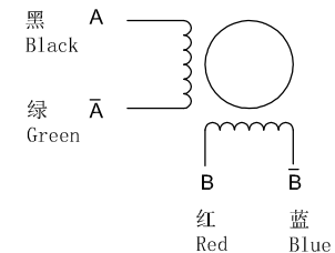
接线图/Connection
